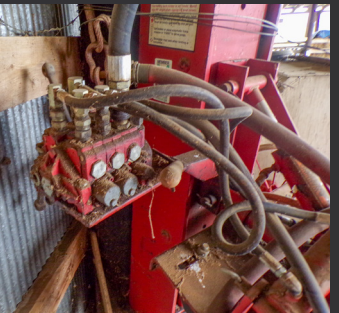
SHAVER POST DRIVER HYDRAULIC 10 INCH
